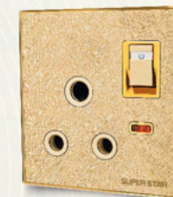
3-Pin Round Socket With Switch & Neon Model: UG-15 15A, 250V
